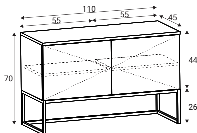
Cabinet 2 doors
