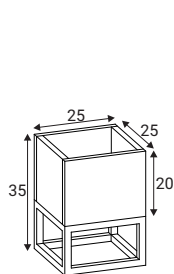
Stawers 1 Stand for flowers
