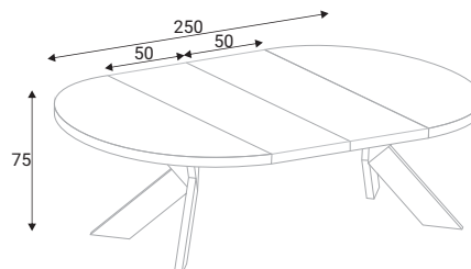
Dining round table D150(250max) + 2 x Extension (150x50)
